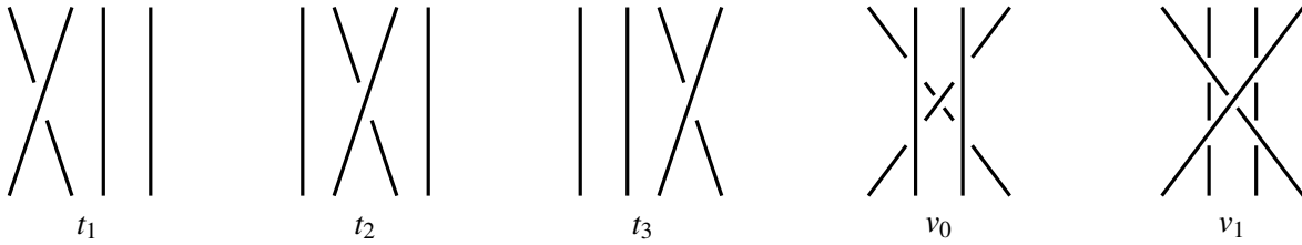
Figure 2.2: Braid pictures of the standard generators t_1, \dots, t_n and elements v_0 and v_1 used in the definition of endomorphisms \alpha_p and \beta_p , depicted here for n = 3 .
