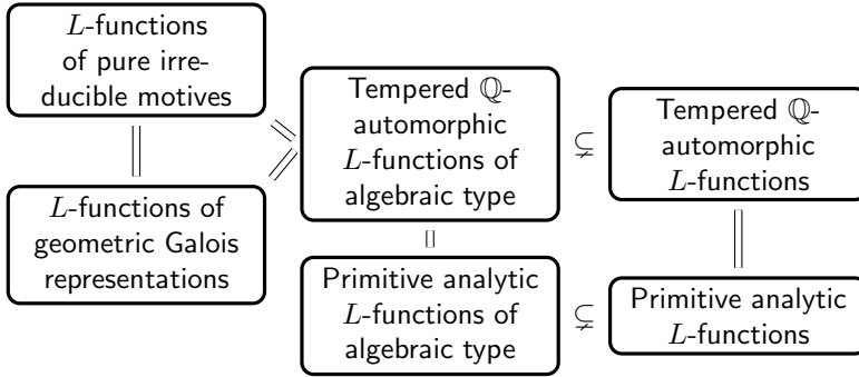
FIGURE 1. Conjectured relationships between the sets of L -functions considered in this paper.
