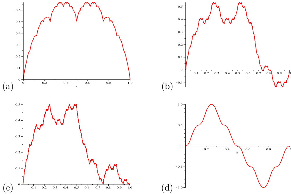
Figure 1: (a) the Takagi function; (b) the Gray Takagi function; (c) Kawamura's T^3 ; (d) a smooth function (see Section 4).
